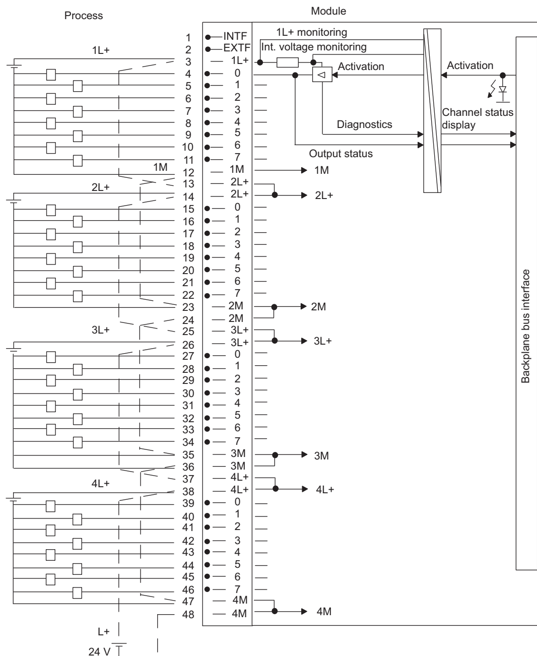
Figure 4-14 Wiring and Block Diagram of the SM 422; DO 32 x DC 24 V/0.5 A
