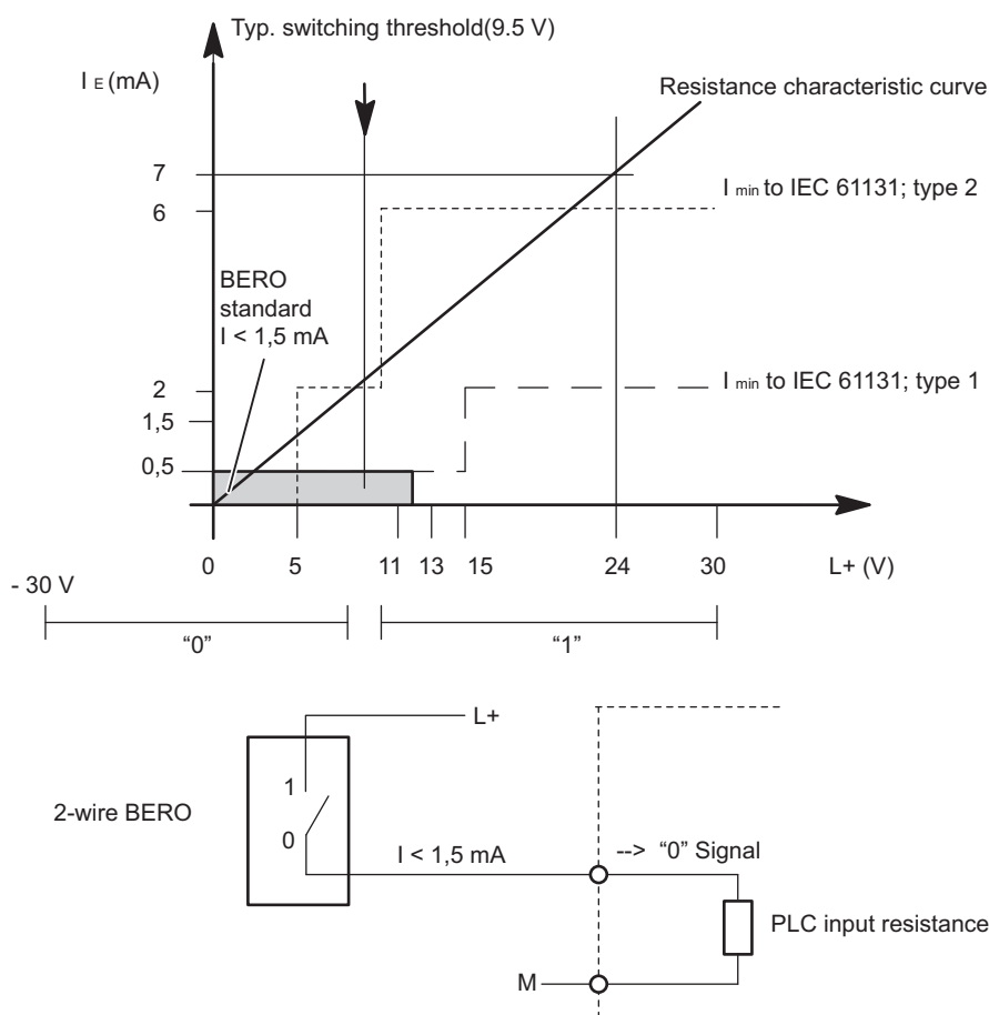
Figure 4-1 Input characteristic curve for digital inputs
