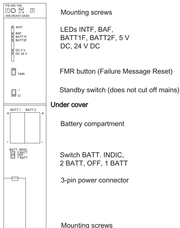
Figure 3-10 Operator Controls and Indicators on the PS 405 10A and the PS 405 10A R
