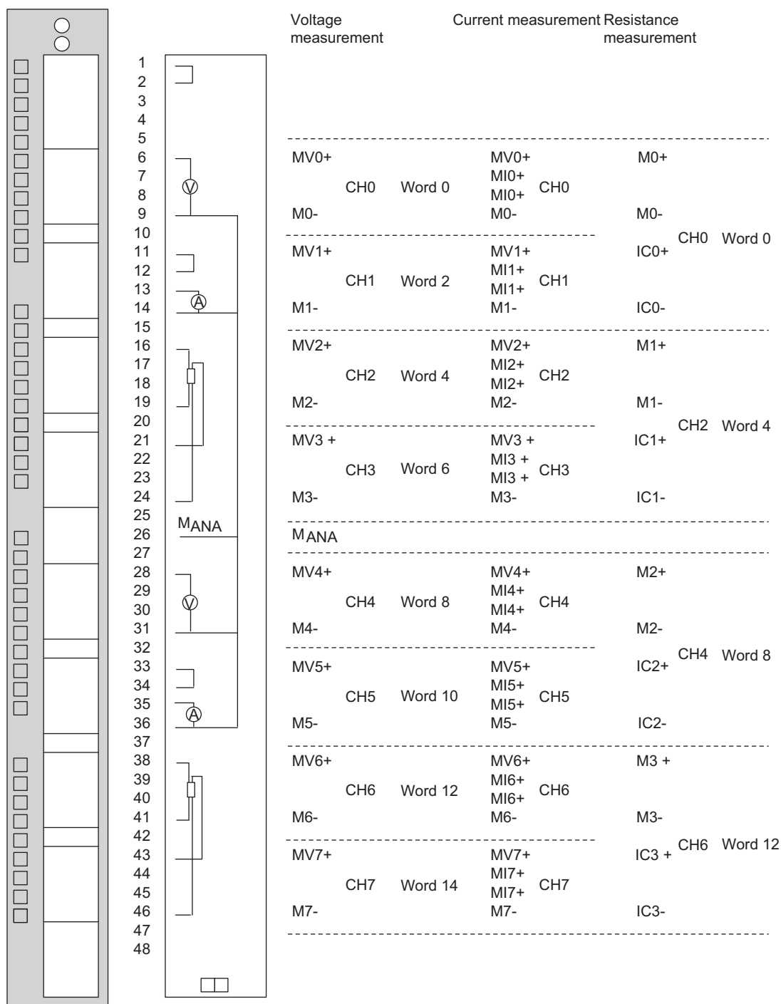
Figure 5-24 Wiring diagram SM 431; AI 8 x 13 Bit
