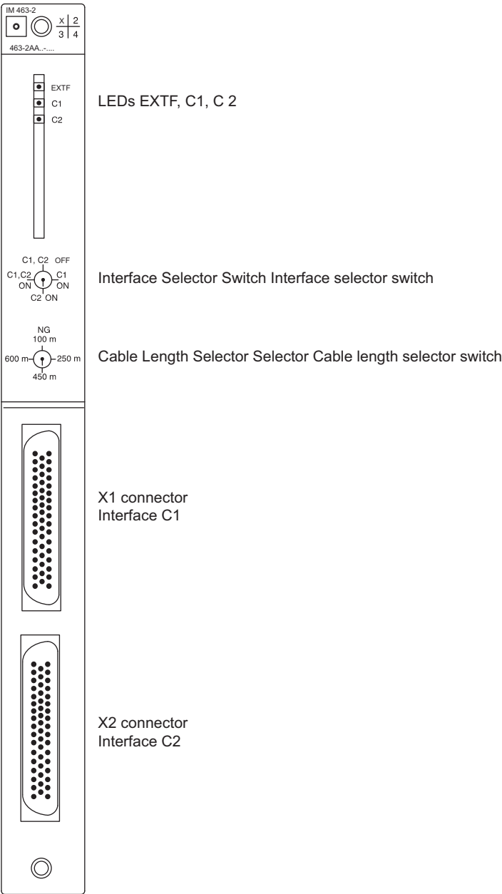
Figure 7-1 Layout of the controls and indicators of the IM 463-2
