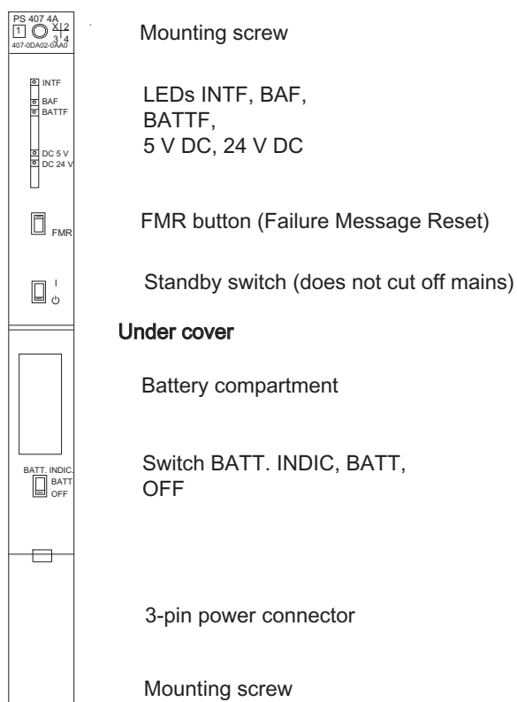
Figure 3-3 Operator controls and indicators on the PS 407 4A
