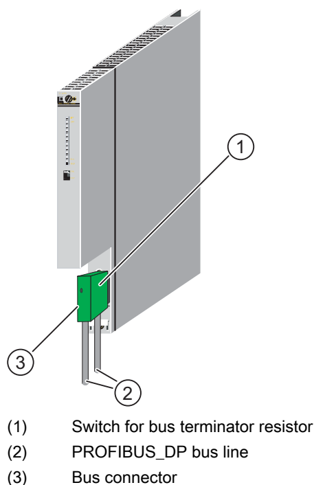
Figure 8-3 Connecting the bus connector to the IM 467
