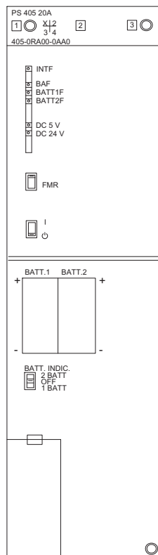
Figure 3-12 Operator controls and indicators on the PS 405 20A
