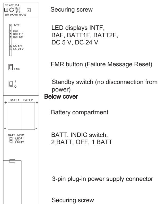
Figure 3-4 Operator controls and indicators of the PS 407 10A and PS 407 10A R
