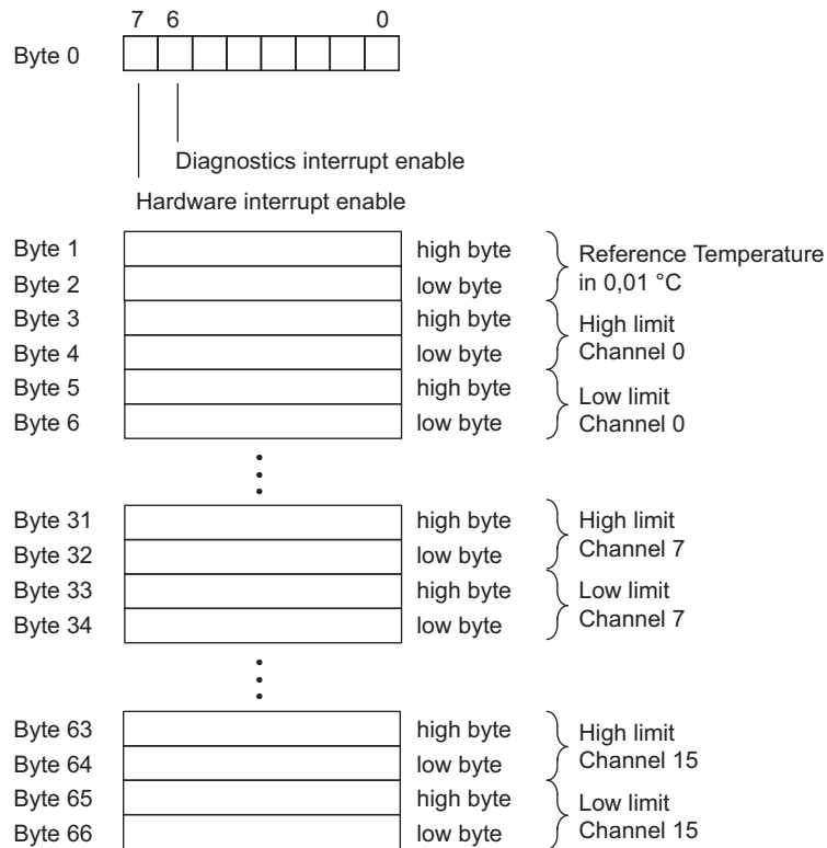
Figure A-2 Data record 1 for the parameters of analog input modules
