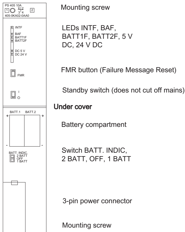
Figure 3-11 Operator Controls and Indicators on the PS 405 10A and the PS 405 10A R
