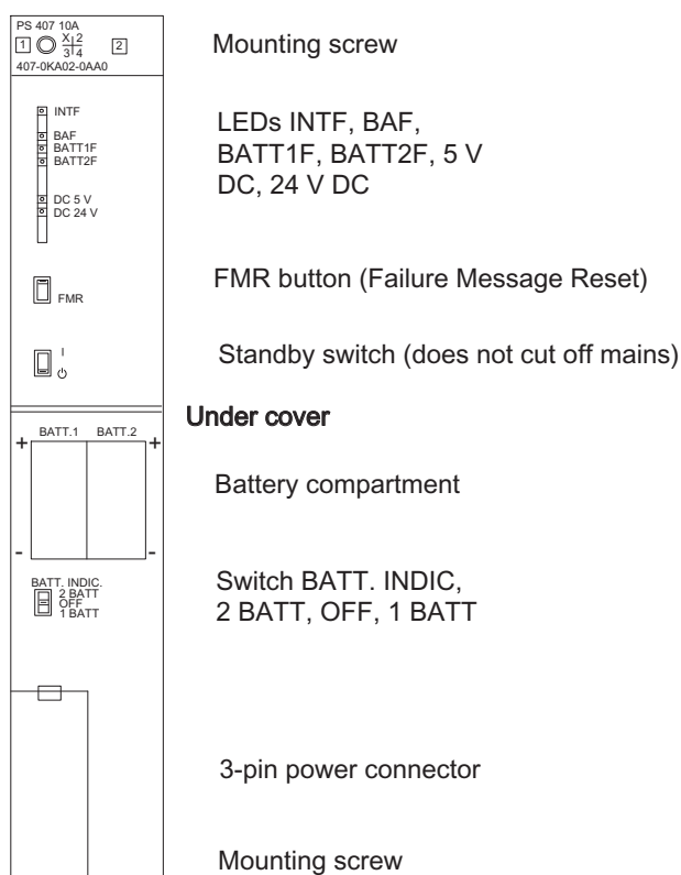
Figure 3-5 Operator controls and indicators of the PS 407 10A and PS 407 10A R
