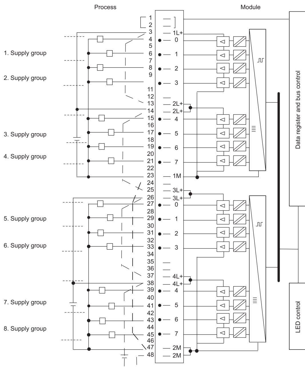
Figure 4-11 Wiring and Block Diagram of the SM 422; DO 16 x DC 24 V/2 A
