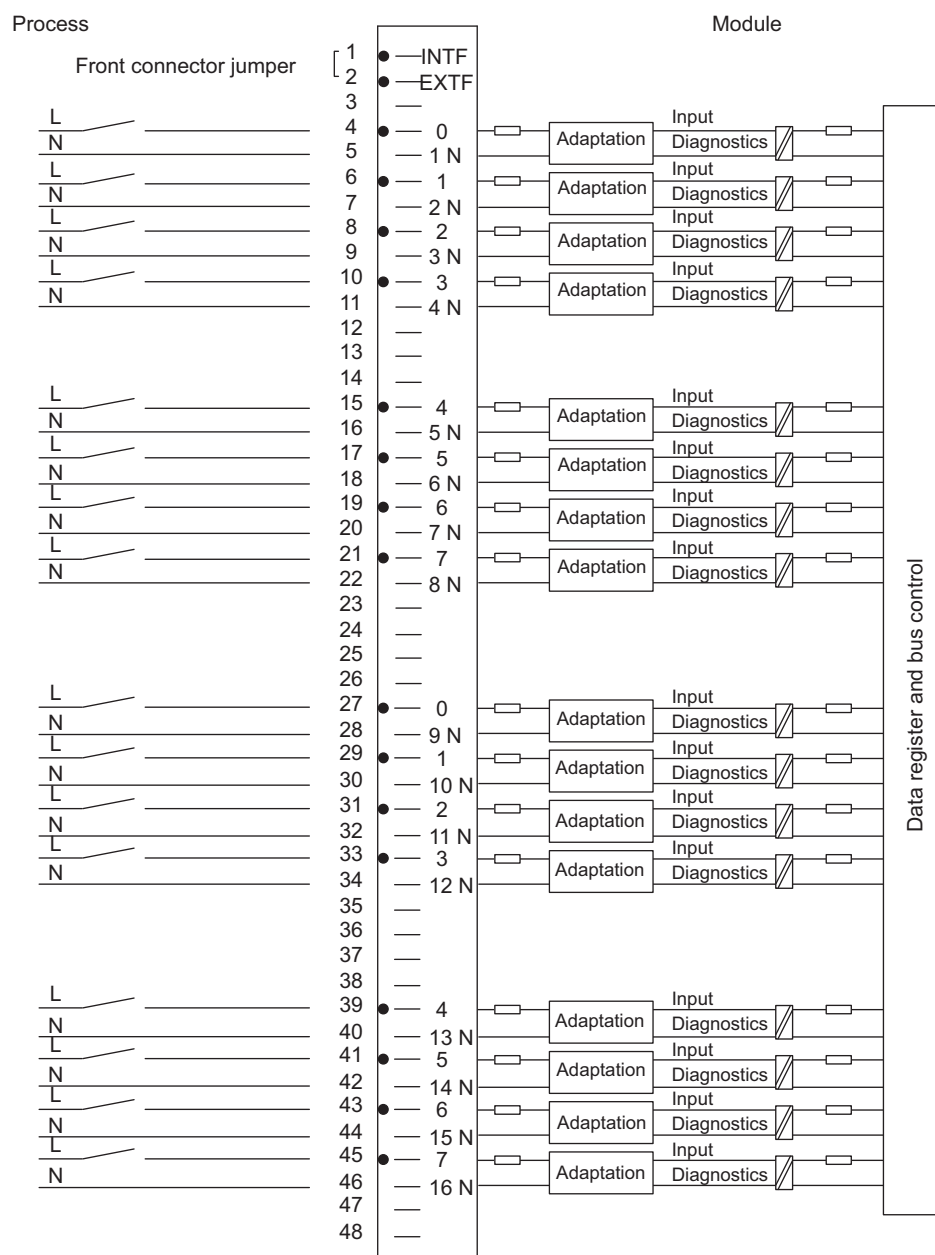
Figure 4-6 Wiring and Block Diagram of the SM 421; DI 16 x UC 24/60 V
