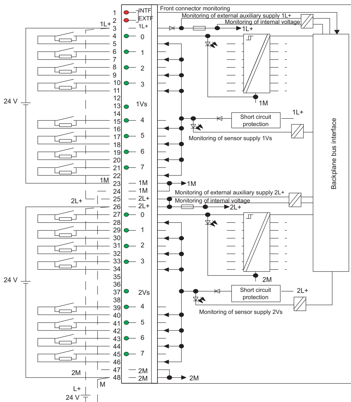
Figure 4-3 Wiring and block diagram of the SM 421; DI 16 x DC 24 V
