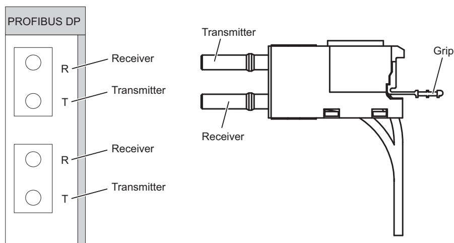
Figure 8-6 Inserting the fiber-optic cables into the IM 467 FO
