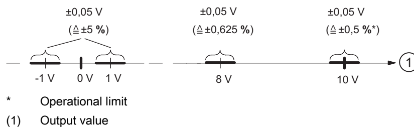
Figure 5-1 Example of the relative error of an analog output module
