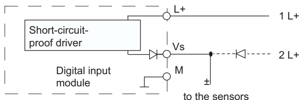
Figure 4-4 Wiring diagram for the redundant supply of sensors of the SM 421; DI 16 x DC 24 V
