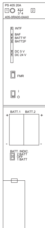
Figure 3-13 Operator controls and indicators on the PS 405 20A
