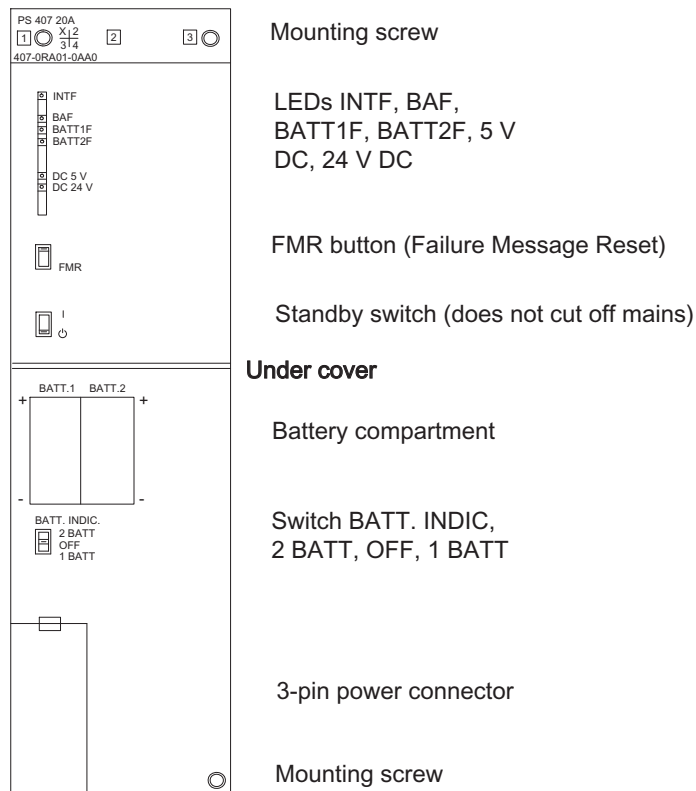
Figure 3-6 Operator controls and indicators on the PS 407 20 A
