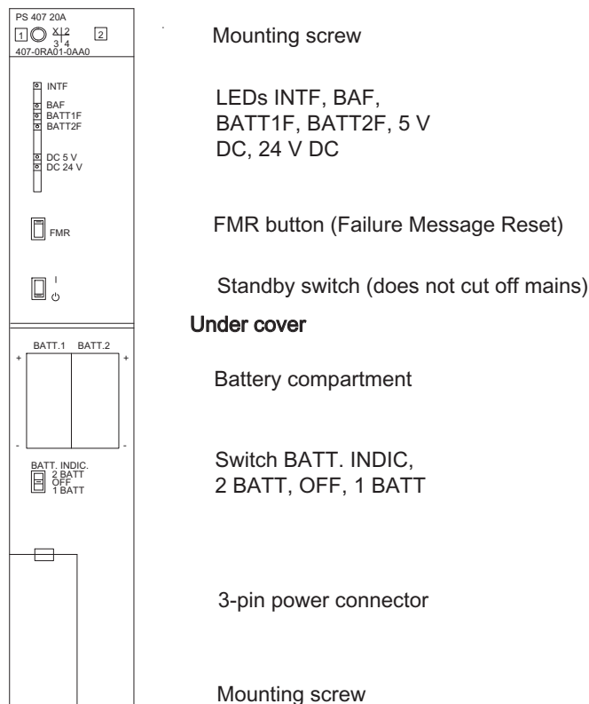
Figure 3-7 Operator controls and indicators on the PS 407 20A power supply module
