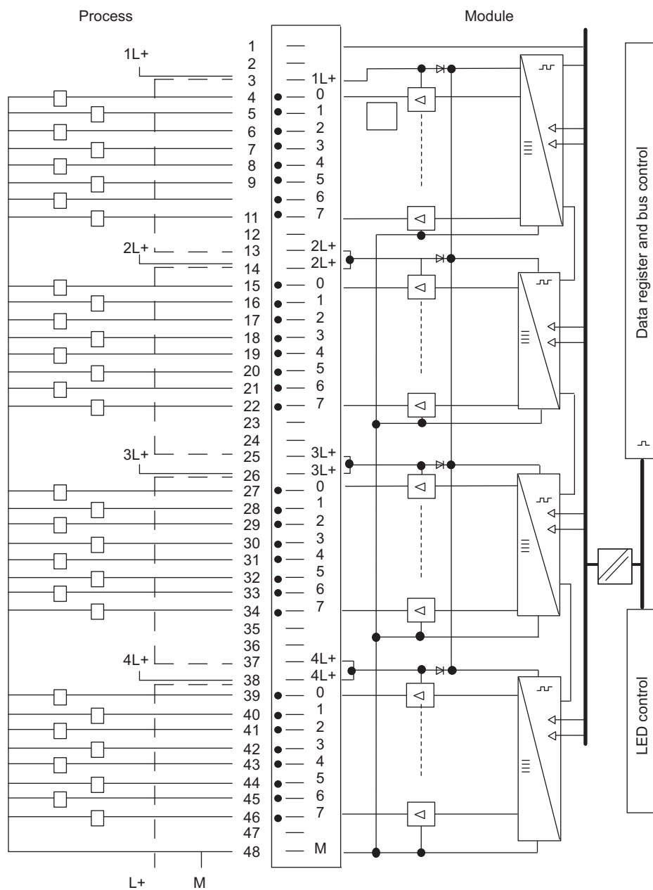
Figure 4-13 Wiring and Block Diagram of the SM 422; DO 32 x DC 24 V/0.5 A
