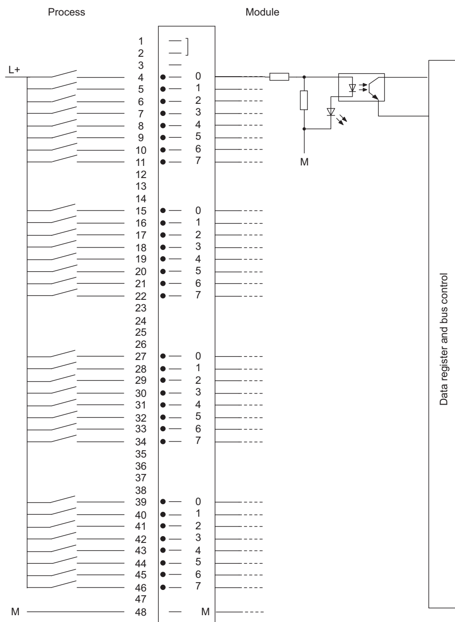
Figure 4-2 Wiring and block diagram of the SM 421; DI 32 x DC 24 V
