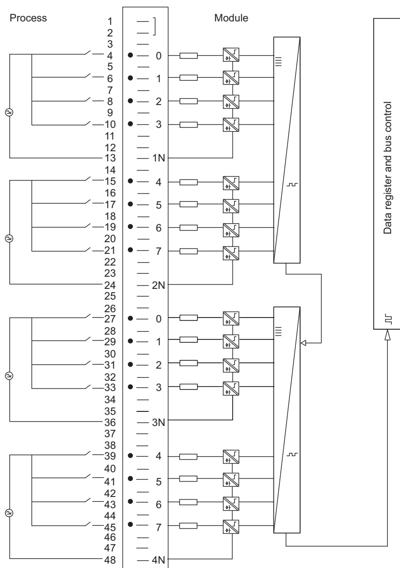
Figure 4-9 Wiring and block diagram of the SM 421; DI 16 x UC 120/230 V
