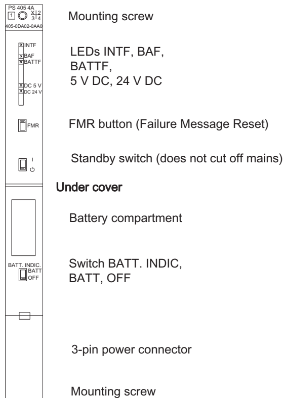
Figure 3-9 Operator controls and indicators on the PS 405 4A
