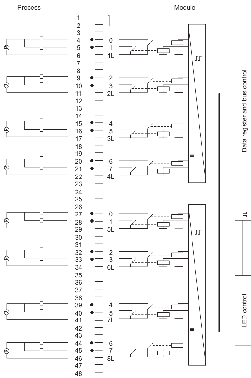
Figure 4-18 Wiring and block diagram of the SM 422; DO 16 x UC 30/230 V/Rel. 5 A
