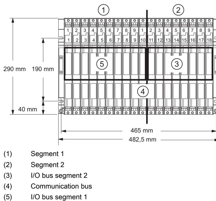
Figure 2-4 CR2 rack
